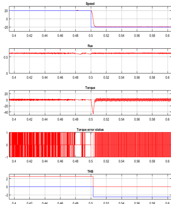
Fig. 13. SIMULATION RESULTS FOR DTC-HB2 DRIVE METHOD OF INDUCTION MOTORS AT RPM SPEEDS OF 20 AND -20 UNDER LIGHT LOAD
