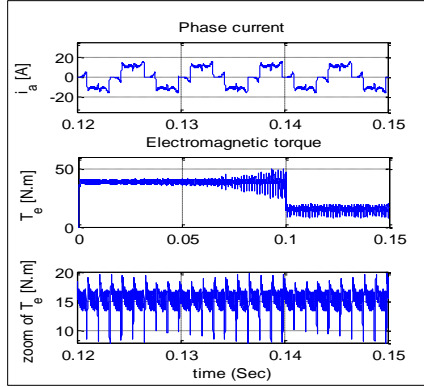
Fig. 8. SIMULATION RESULTS OF DIRECT TORQUE CONTROL METHOD BASED ON TWO-PHASE CONDUCTION FOR NON-IDEAL PMBL MOTOR
