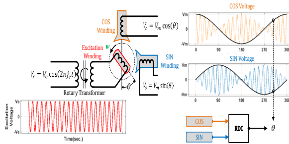
Fig.1. BASIC STRUCTURE OF A TYPICAL 2-POLE ROTARY RESOLVER
